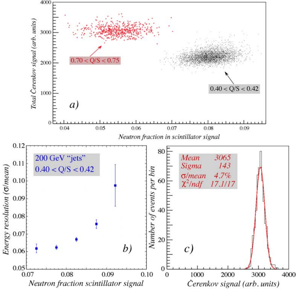
Figure 20: Scatter plot for 200 GeV “jet” events, all of which had either a Q/S signal ratio between 0.40 and 0.42 (the black dots), or between 0.70 and 0.75 (the red crosses). For each individual event, the combination of the total Čerenkov signal and the fractional contribution of neutrons to the total scintillator signal is given (a). The energy resolution for 200 GeV “jets” with the same em shower fraction, as a function of the fractional neutron contribution to the scintillator signals (b). Čerenkov signal distribution for 200 GeV “jets” with 0.70 < Q/S < 0.75 and 0.45 < f_n < 0.65 , together with the results of a Gaussian fit (c) [9].
